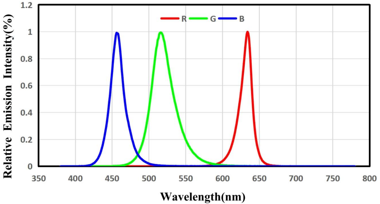
Radiation Characteristics
