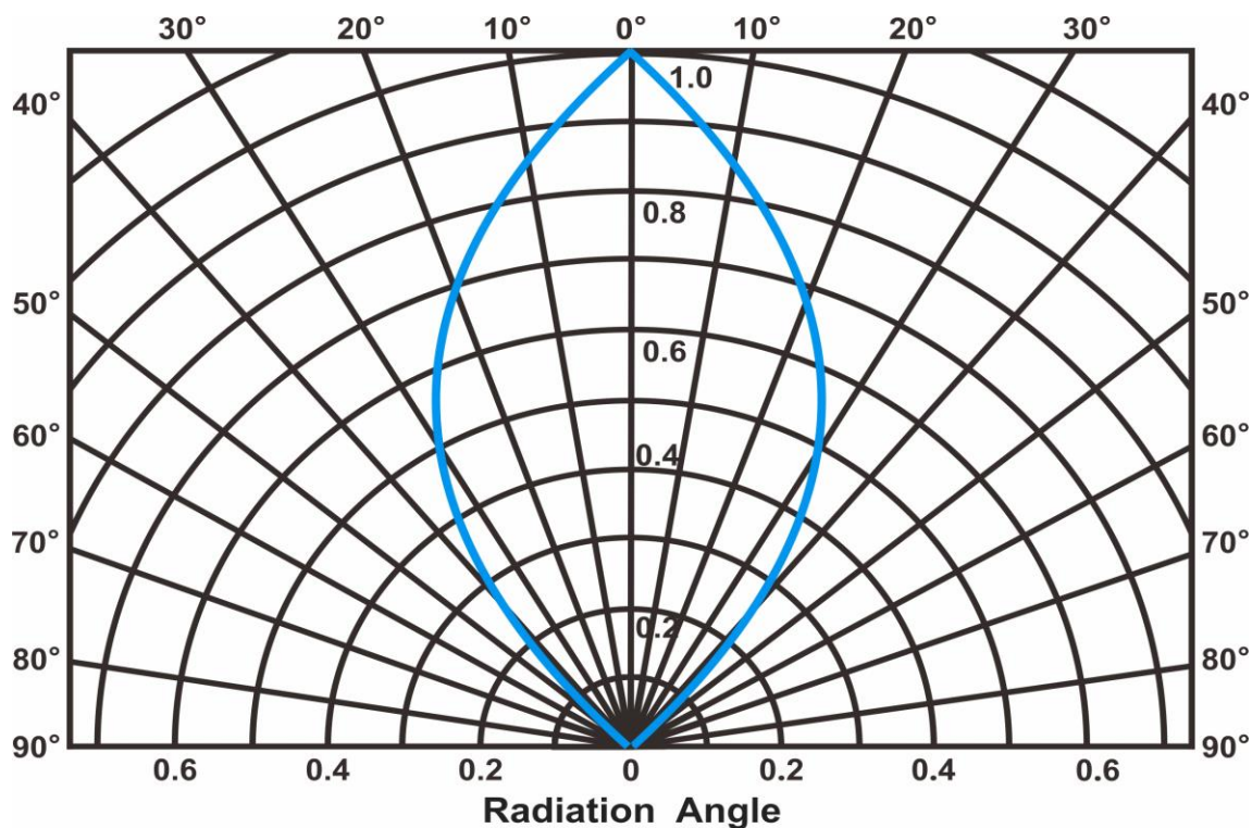
Radiation Characteristics
