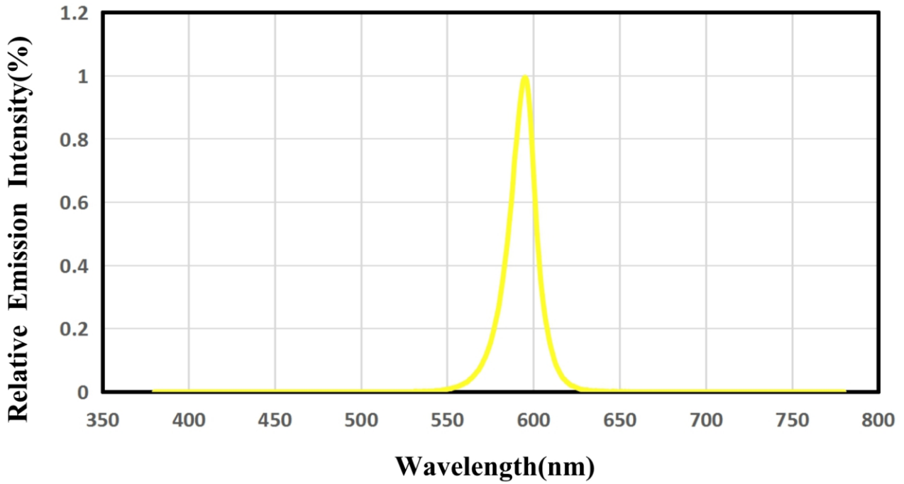
Radiation Characteristics
