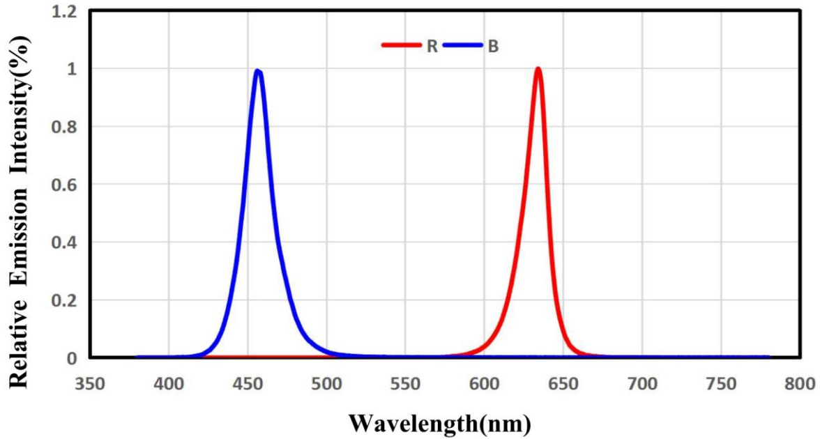
Radiation Characteristics
