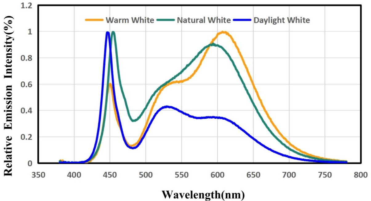
Radiation Characteristics
