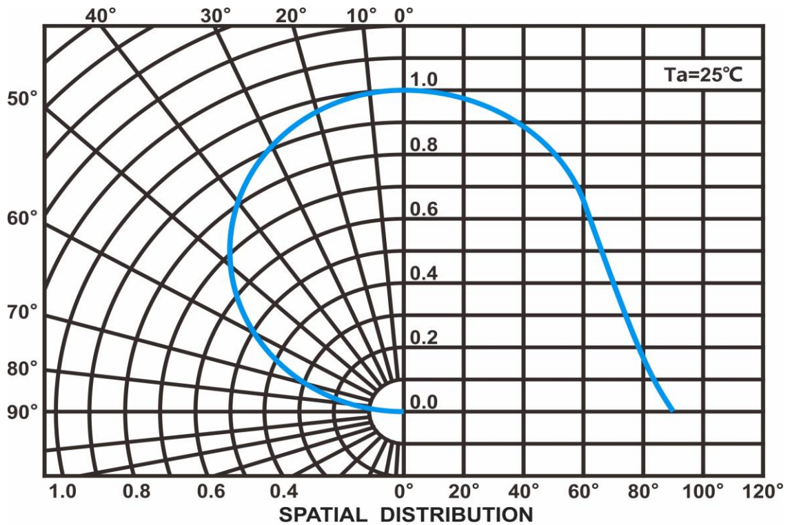
Radiation Characteristics
