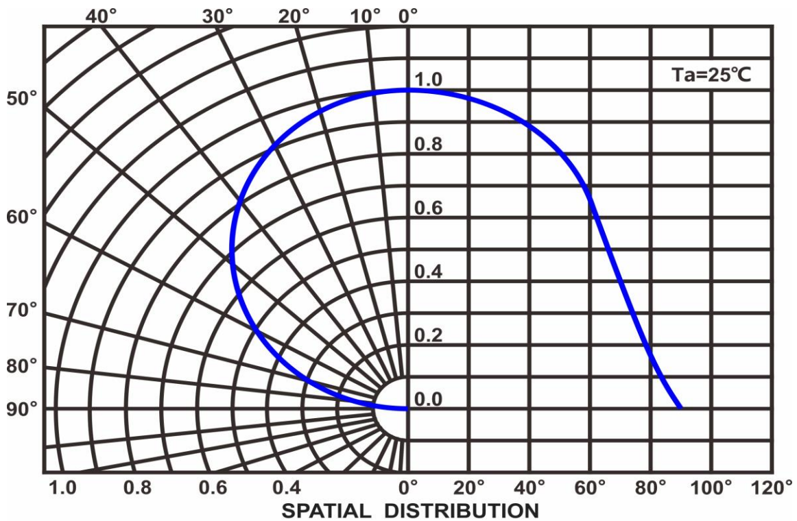
Radiation Characteristics
