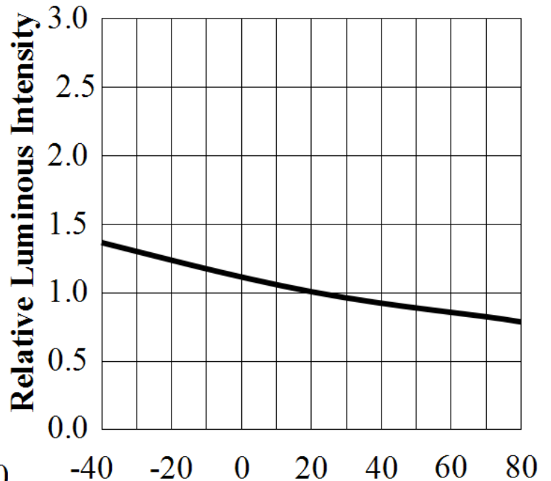
Relative Intensity VS. Ambient Temperature
