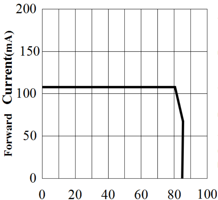
Allowable Forward Current VS. Ambient Temperature
