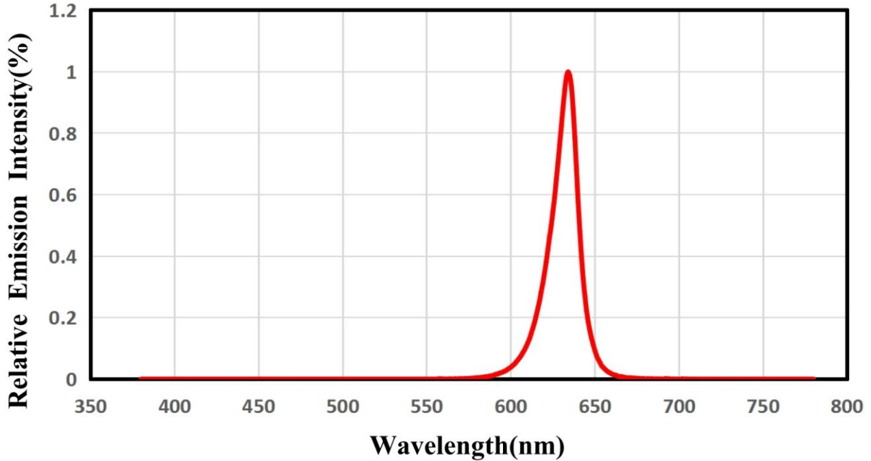
Radiation Characteristics
