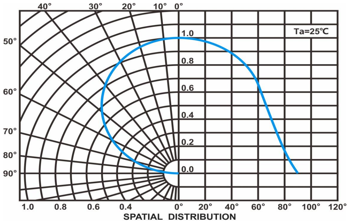
Radiation Characteristics
