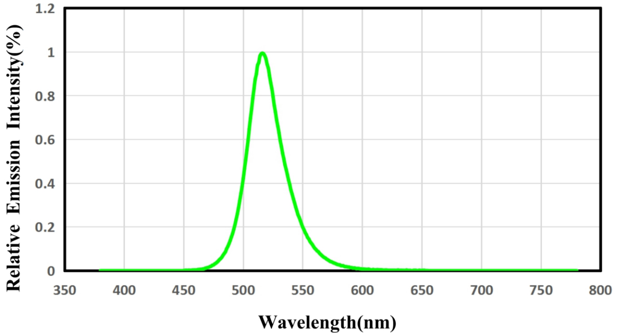
Radiation Characteristics
