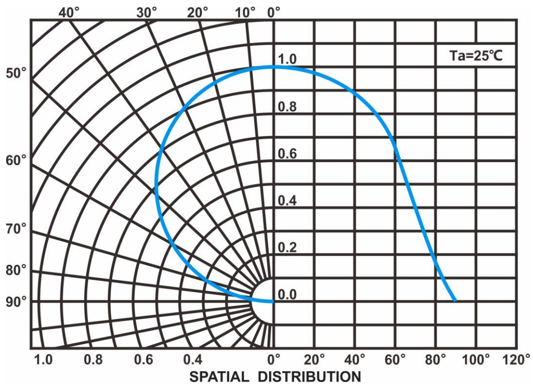
Radiation Characteristics
