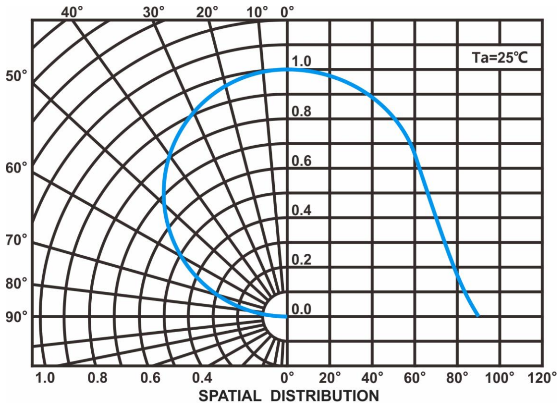
Radiation Characteristics
