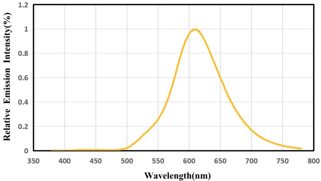
Radiation Characteristics
