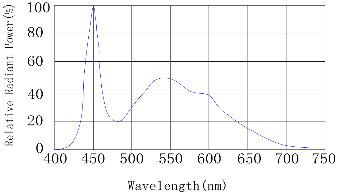
Radiation Characteristics
