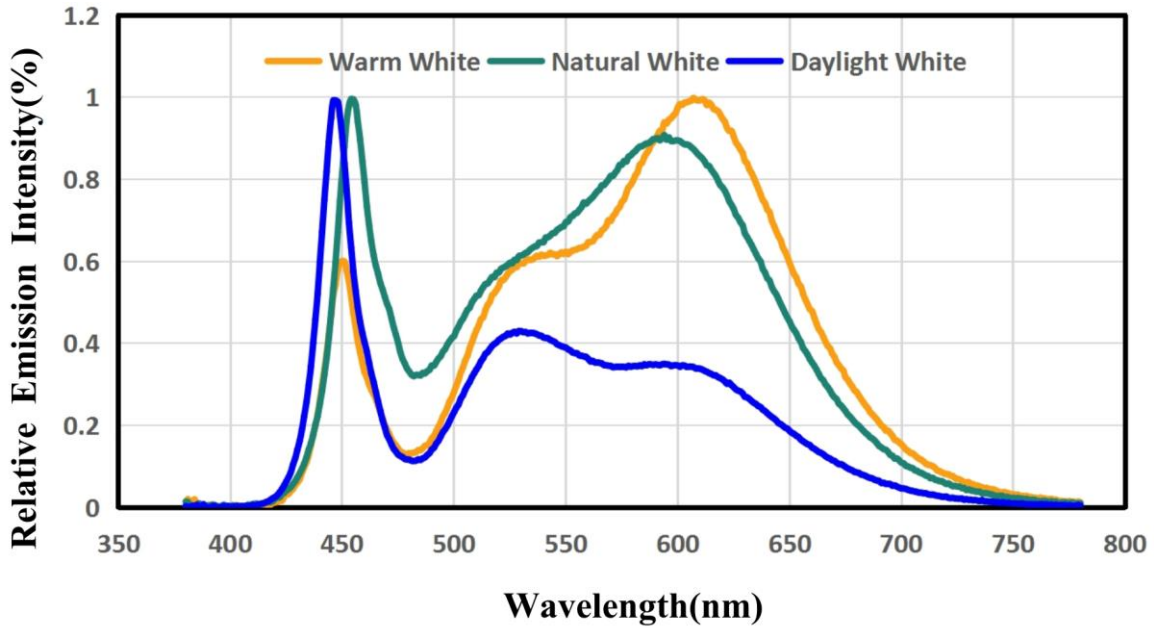
Radiation Characteristics
