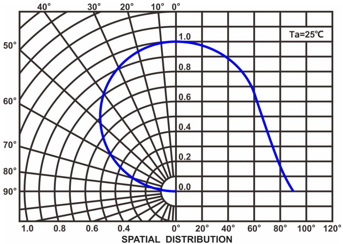
Radiation Characteristics
