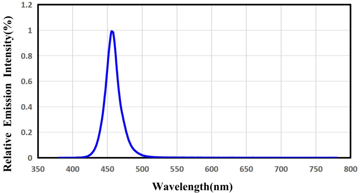
Radiation Characteristics
