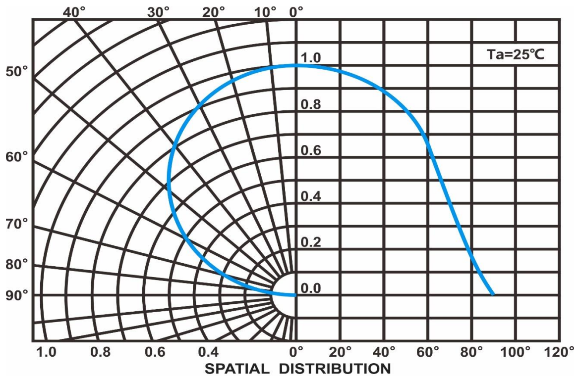
Radiation Characteristics
