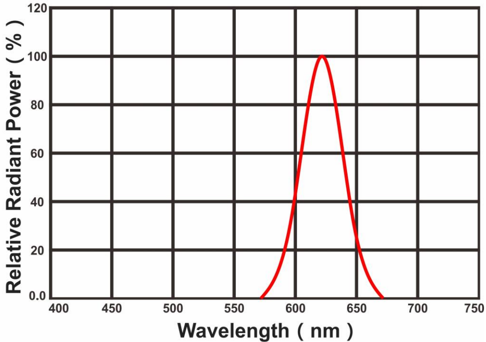
Radiation Characteristics
