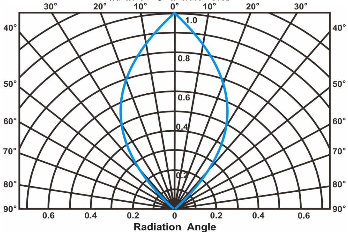
Radiation Characteristics
