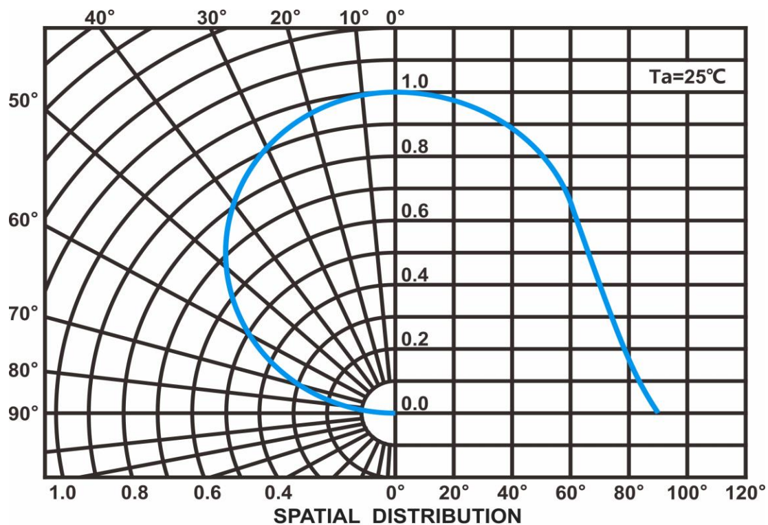
Radiation Characteristics
