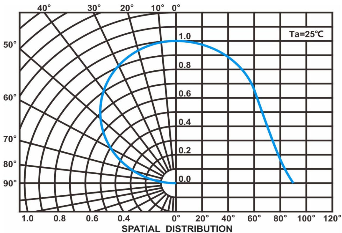
Radiation Characteristics
