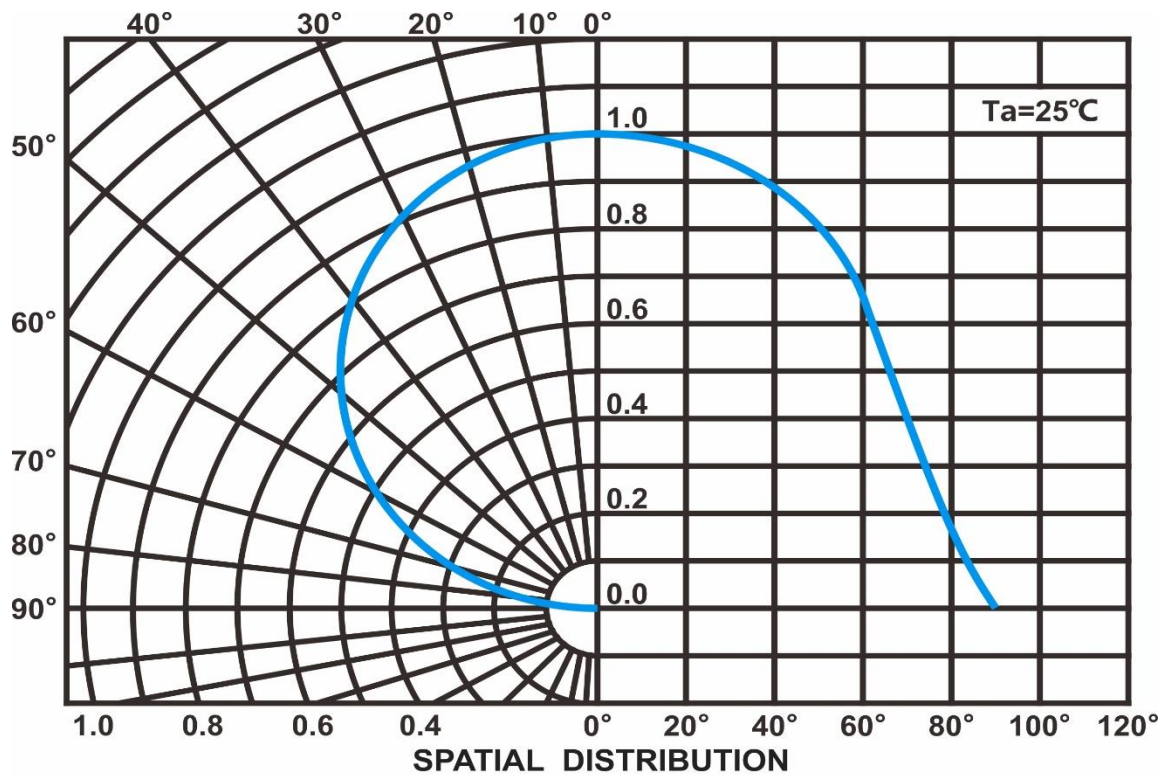
Radiation Characteristics
