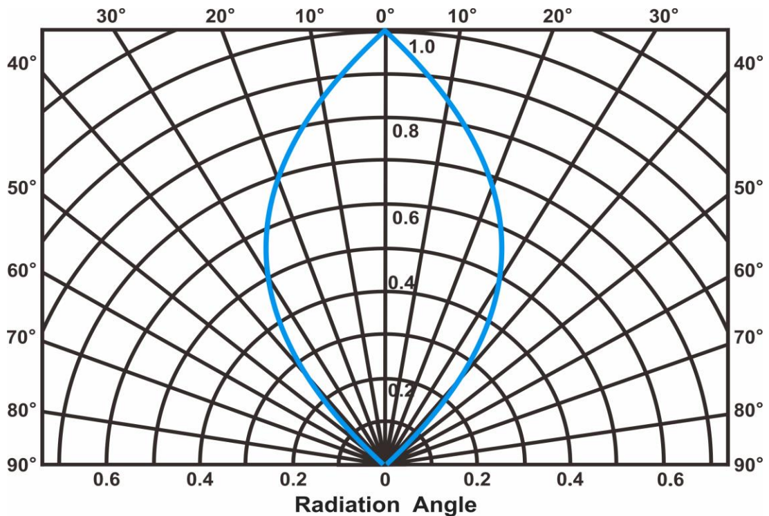
Radiation Characteristics
