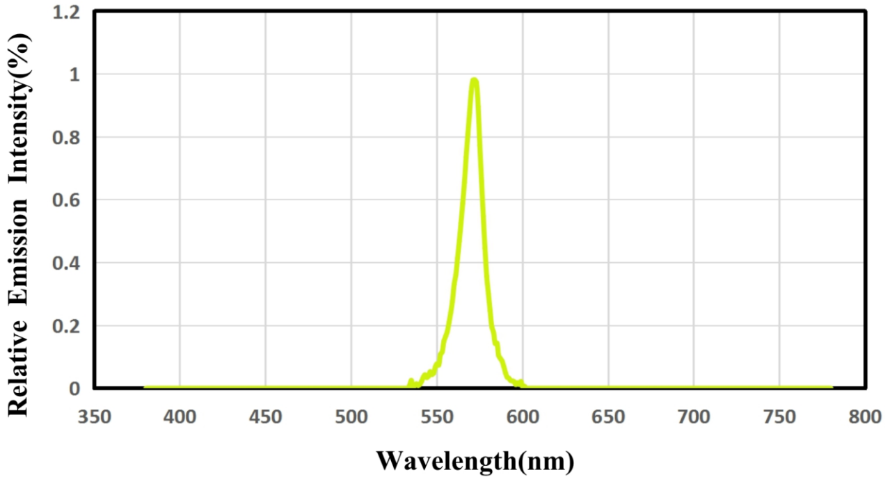
Radiation Characteristics
