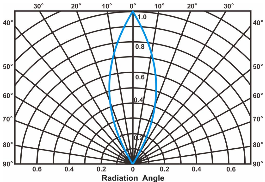
Radiation Characteristics
