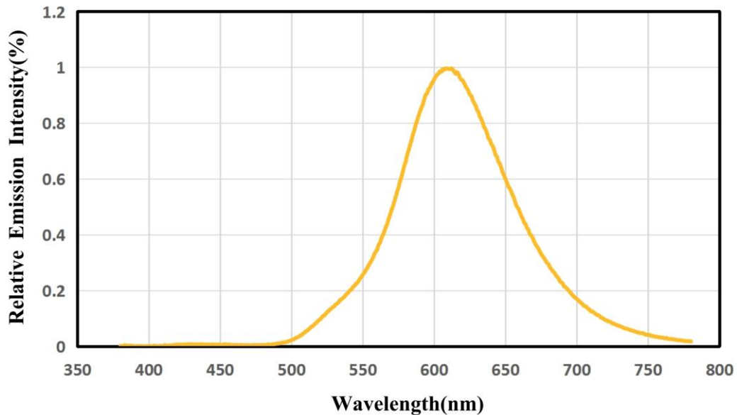
Radiation Characteristics
