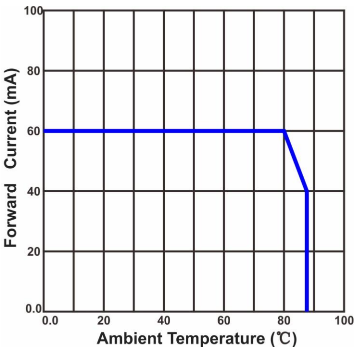
Allowable Forward Current VS. Ambient Temperature
