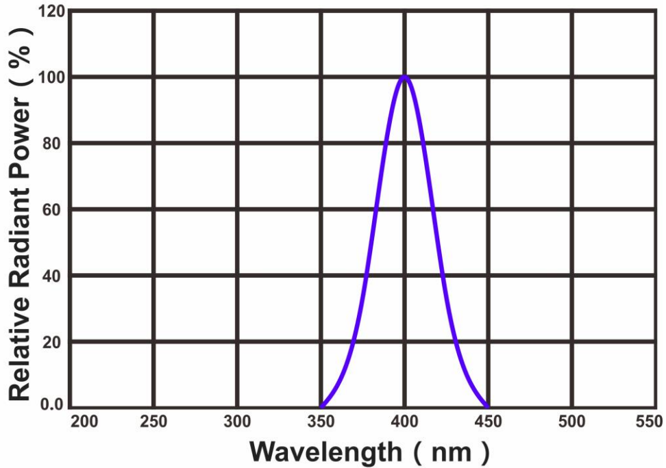
Radiation Characteristics
