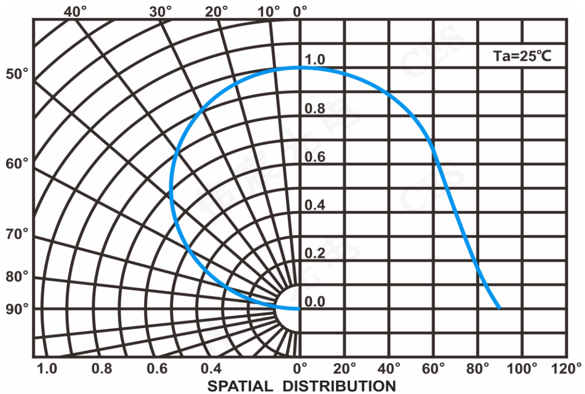
Radiation Characteristics
