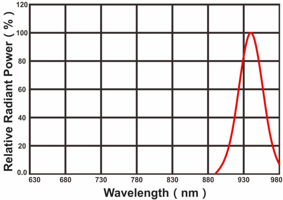
Radiation Characteristics
