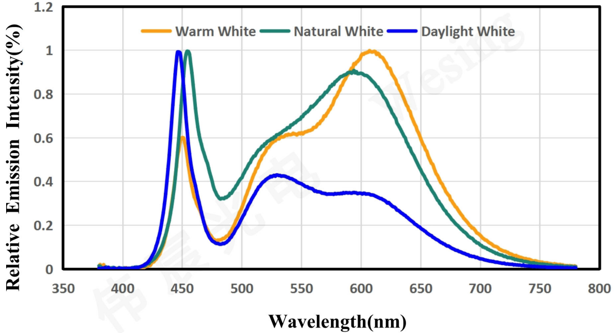
Radiation Characteristics
