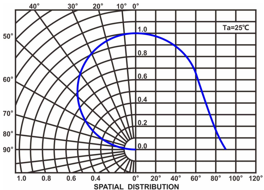
Radiation Characteristics
