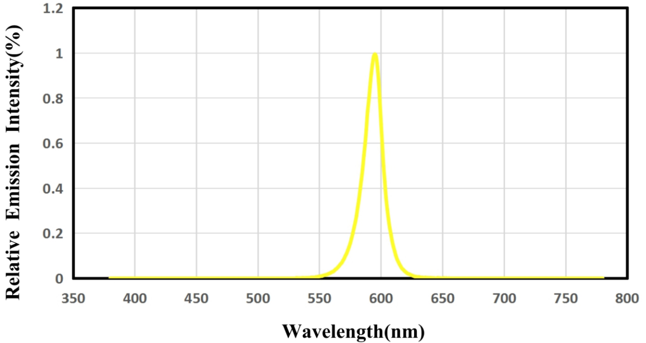
Radiation Characteristics
