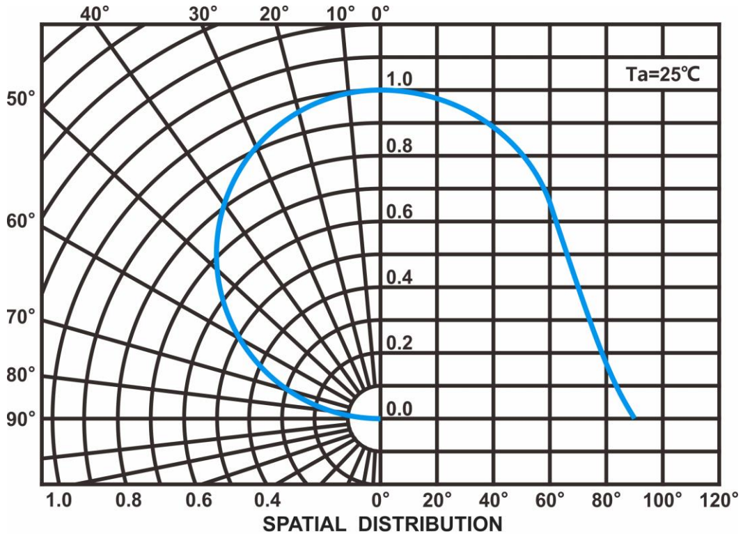
Radiation Characteristics
