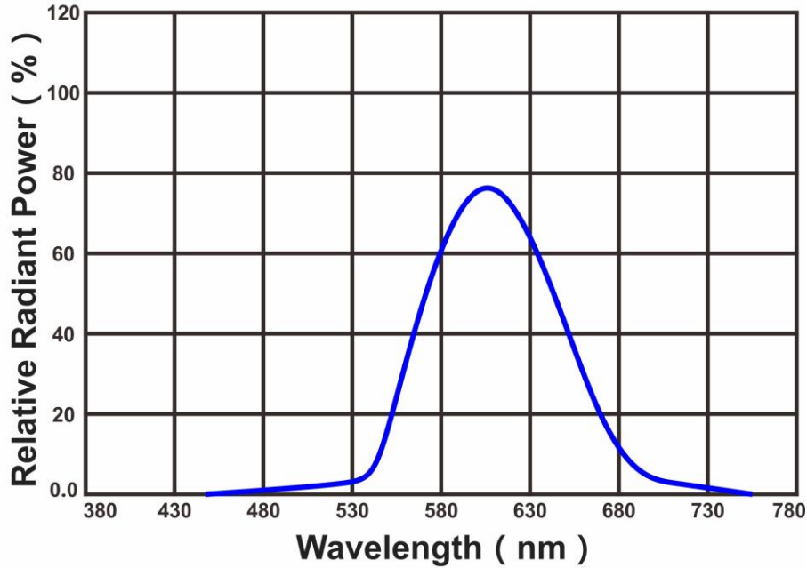
Radiation Characteristics
