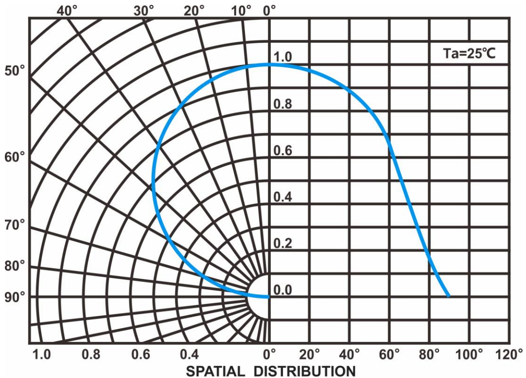
Radiation Characteristics
