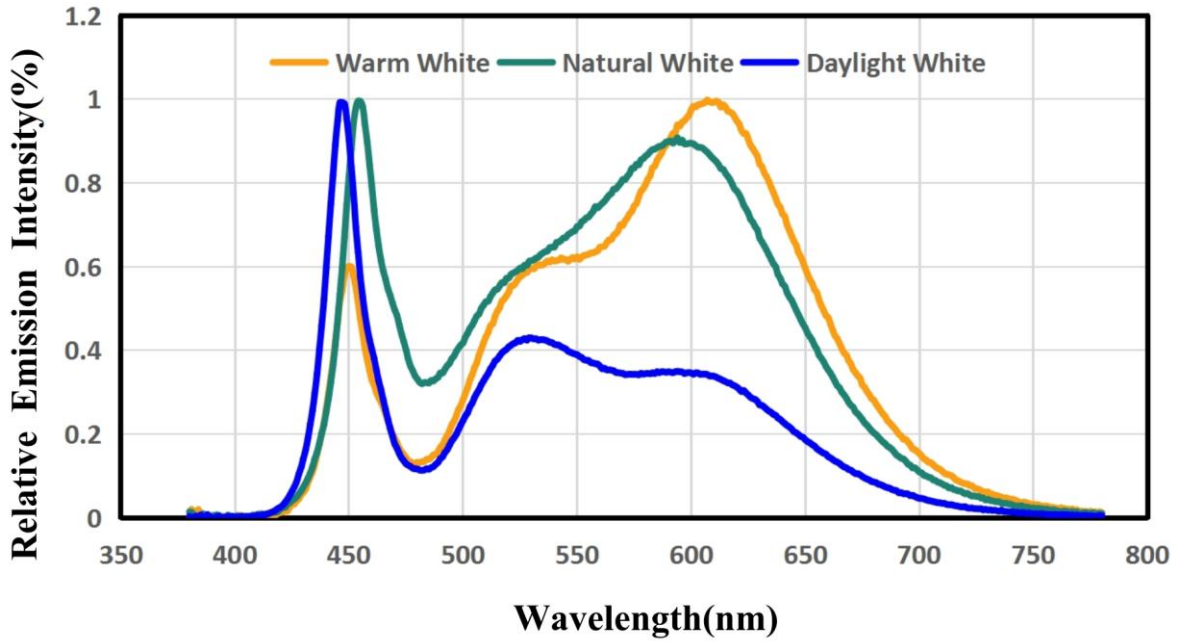
Radiation Characteristics
