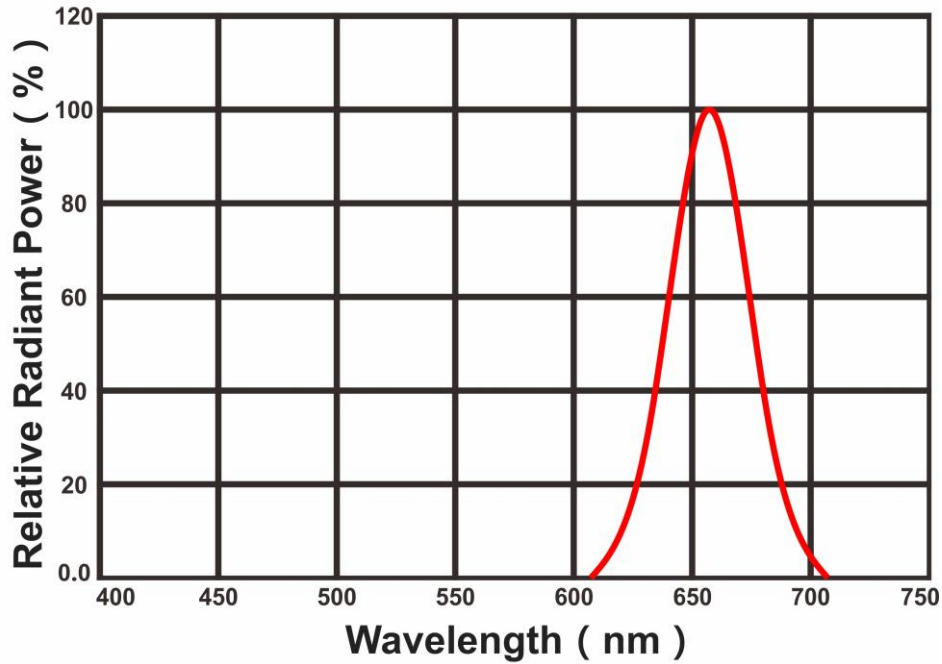
Radiation Characteristics
