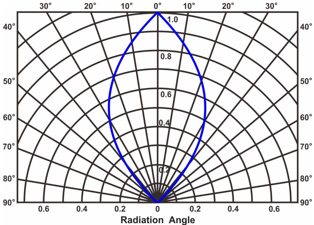
Radiation Characteristics
