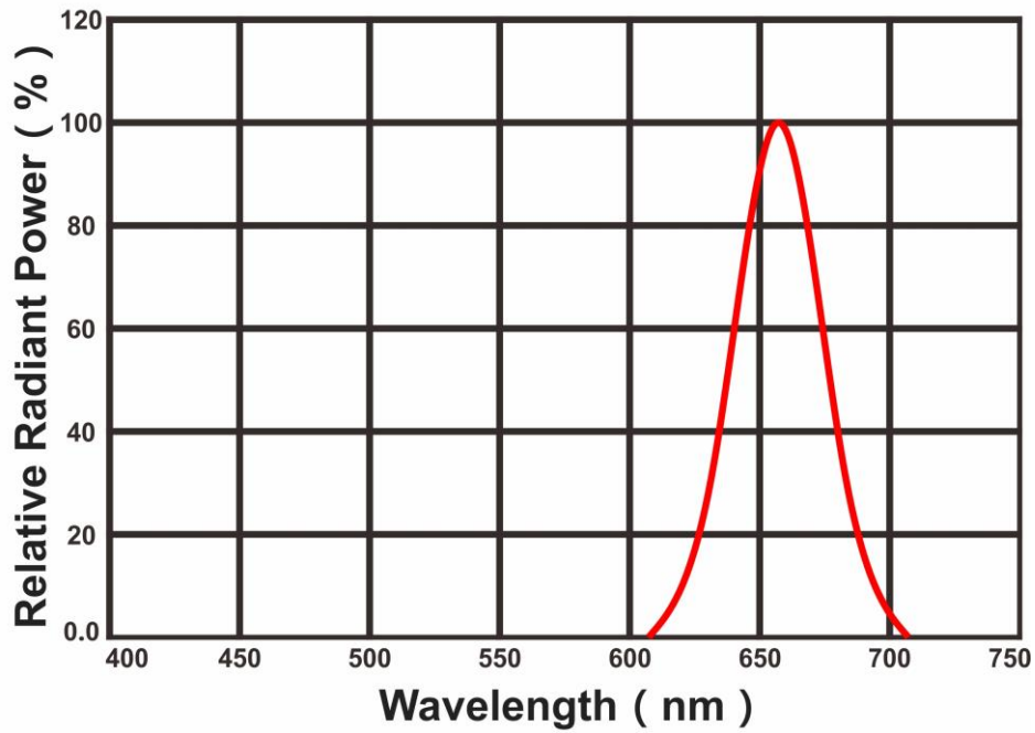
Radiation Characteristics
