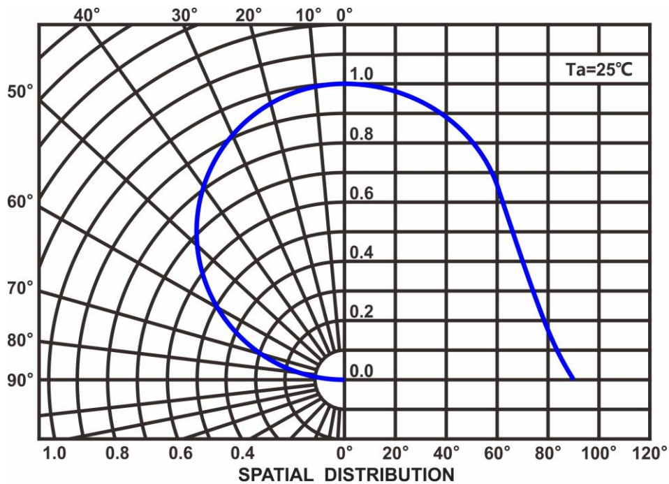
Radiation Characteristics
