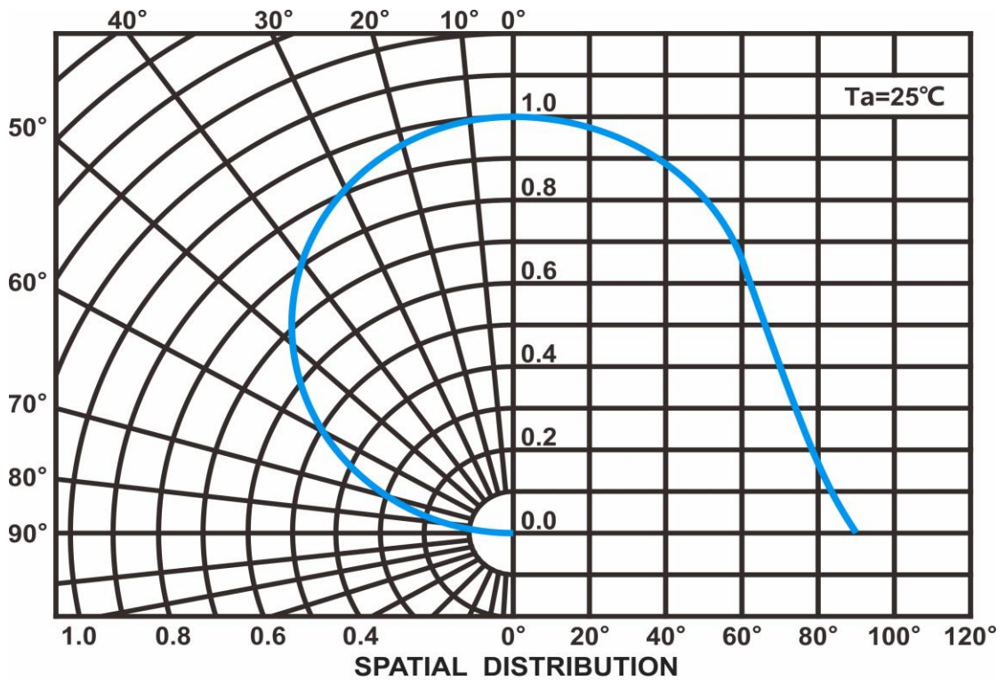
Radiation Characteristics
