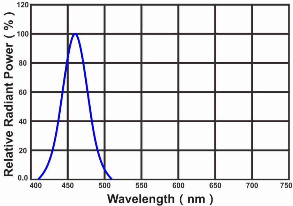
Radiation Characteristics
