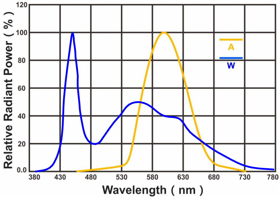
Radiation Characteristics
