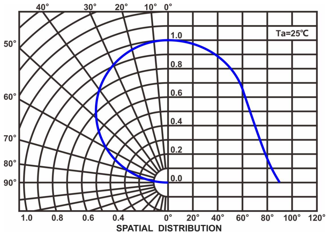
Radiation Characteristics
