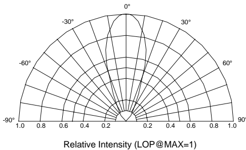
Beam Pattern
