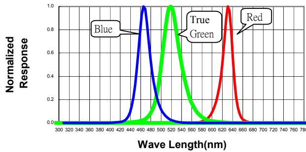
Spectral Radiance True Green Peak @ 515nm Red Peak @ 630nm Blue Peak @ 468nm
