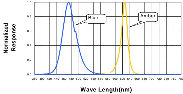
Spectral Radiance Amber Peak @ 605nm Blue Peak @ 468nm
