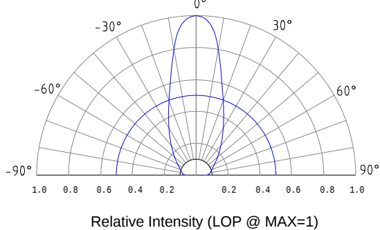
Beam Pattern
