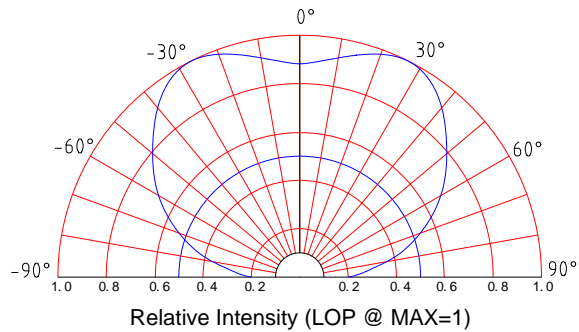
Beam Pattern
